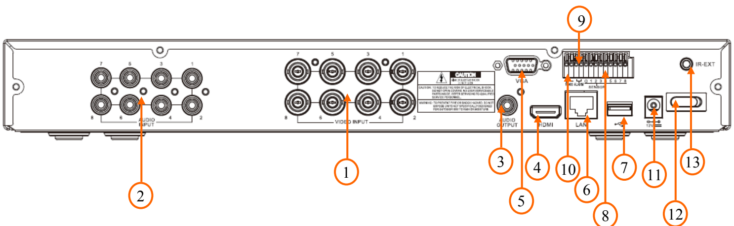
NHDR-5208AHD
