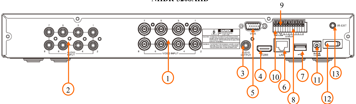
NHDR-5208AHD
