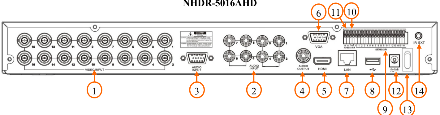
NHDR-5016AHD
