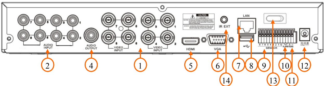
NHDR-5008AHD
