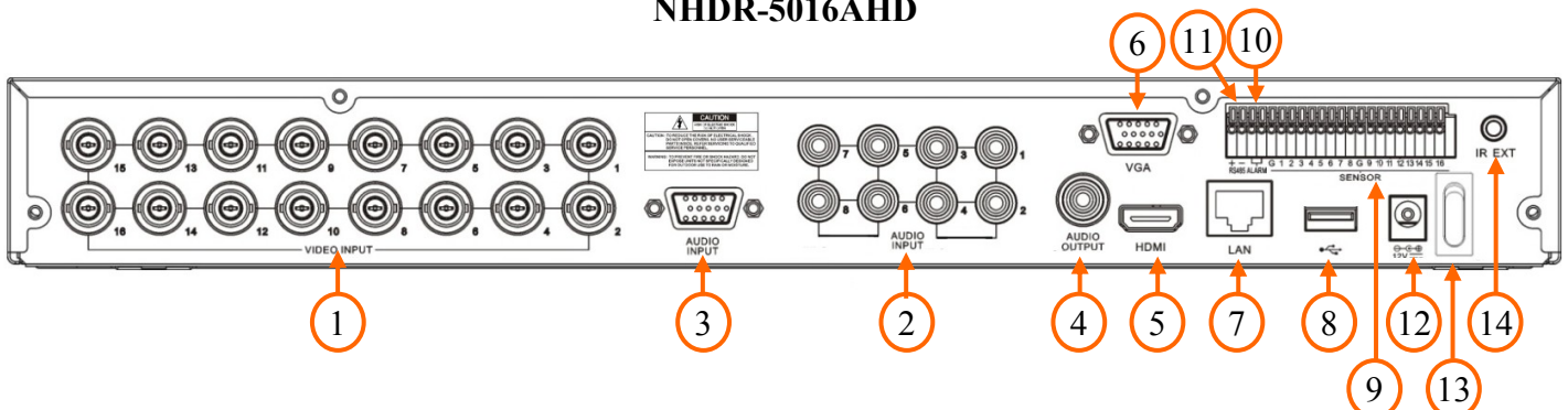
NHDR-5016AHD
