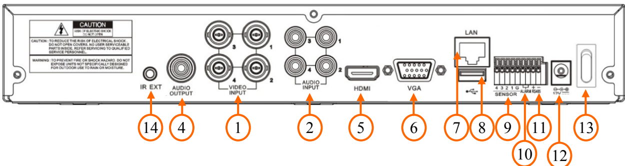
NHDR-5008AHD
