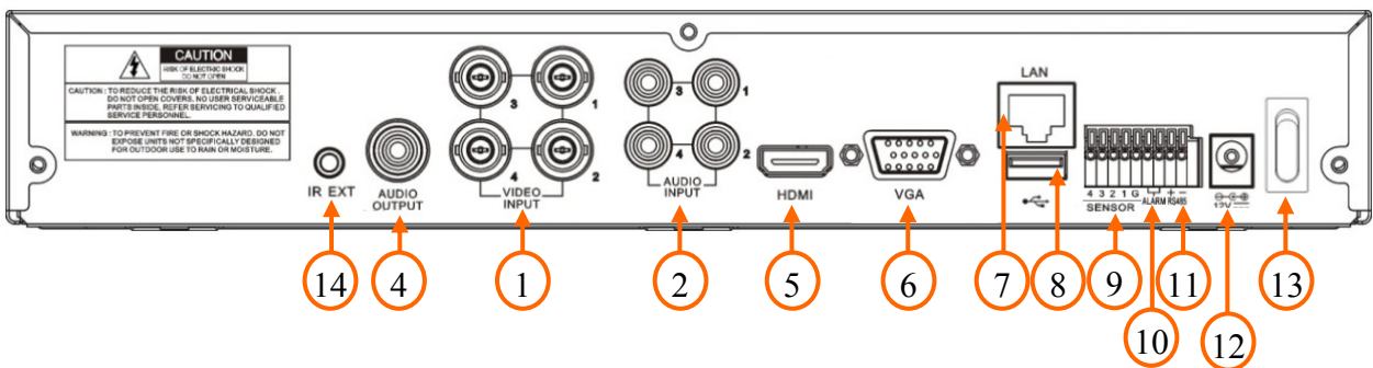
NHDR-5008AHD
