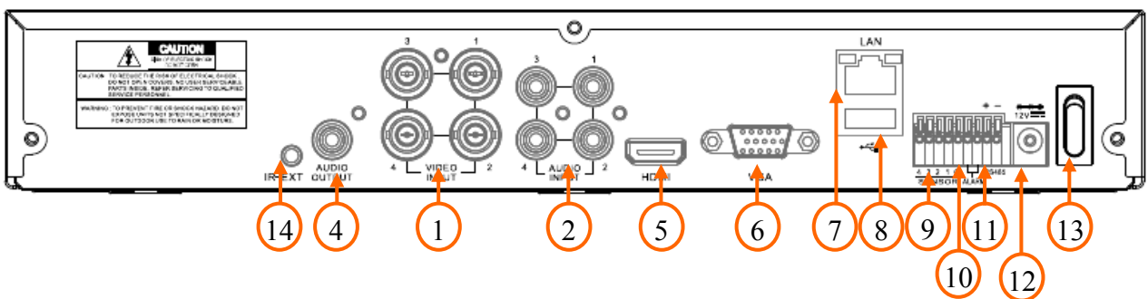
NHDR-5008AHD-II
