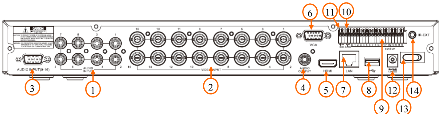
NHDR-5016AHD-II
