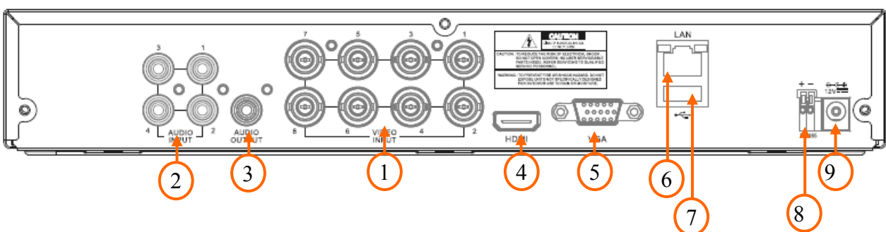
NHDR-3208AHD
