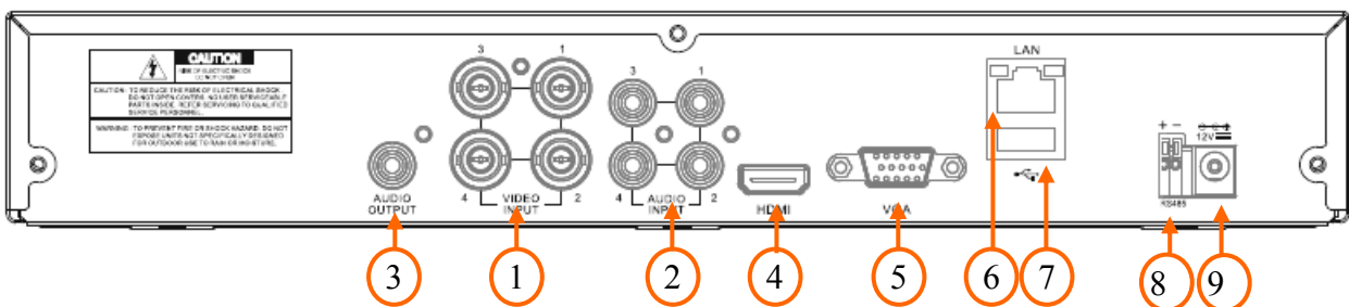
NHDR-3204AHD
