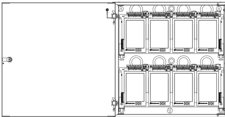
Rys. 5.6.1/4 Centrala P6000-11110-xxxx-xxxx-xxx0x
